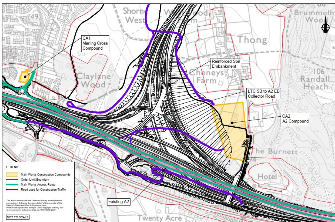
Plate 7.6 Location of reinforced soil embankment
